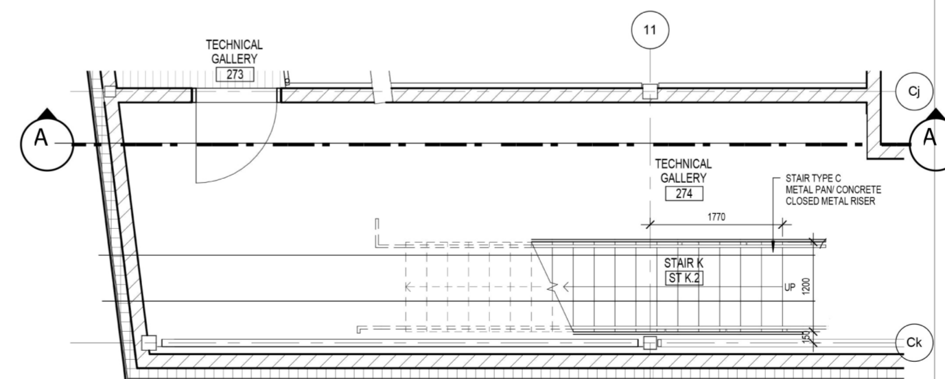
LEVEL 1 PLAN
