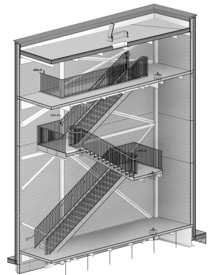
SOUTH VIEW
