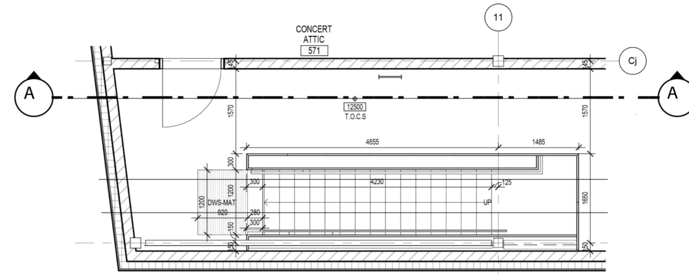
LEVEL 3 PLAN
