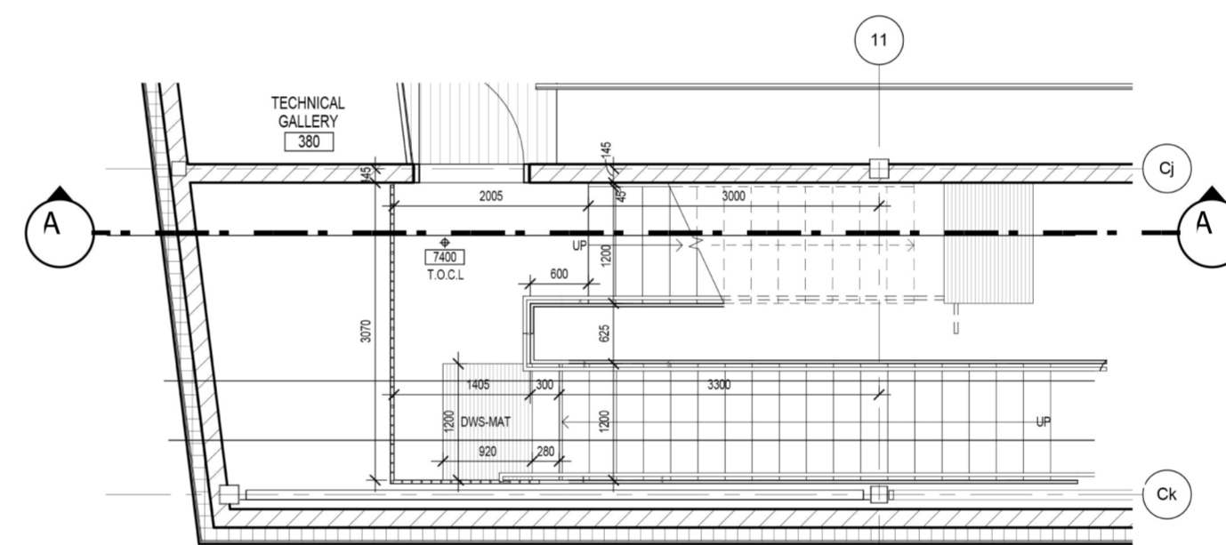
LEVEL 2 PLAN
